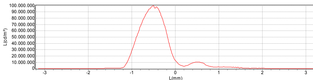
Diagram 6: Projection of arc profile (parallel to line 1 in the area 1.s 20%)
