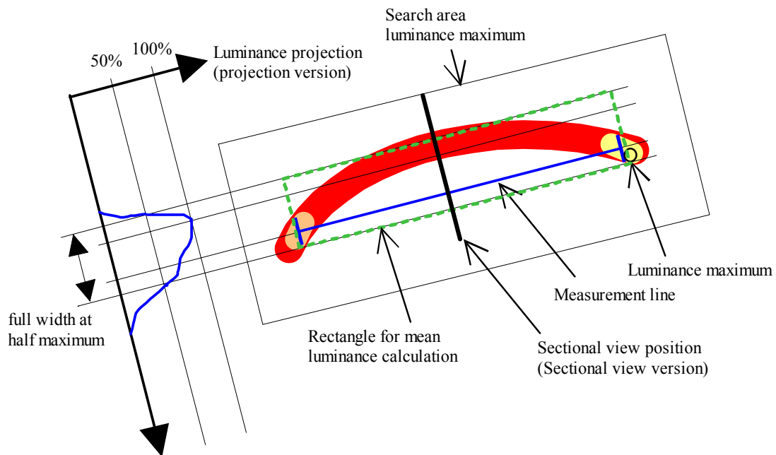
Diagram 4: Specification of arc parameters according to ECE 99
