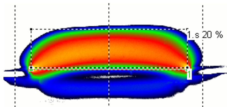
Diagram 5: Luminance image with measuring regions (false color, logarithmic representation)
